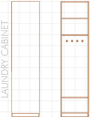
LAUNDRY CABINET FOR USED CLOTHES W - 500-600 @ 10mm interval D - 200-300 @ 10mm interval H - 1950 - 2100 - 2400
