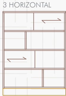
OPEN UNIT SHELVES (3&4) WITH SLIDE SHUTTERS
