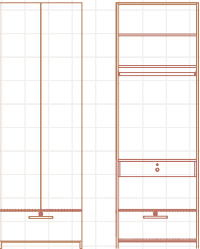
EXTERNAL 1 DRAWER W - 800,900,1000 D - 580 H - 1950 - 2100 - 2400
