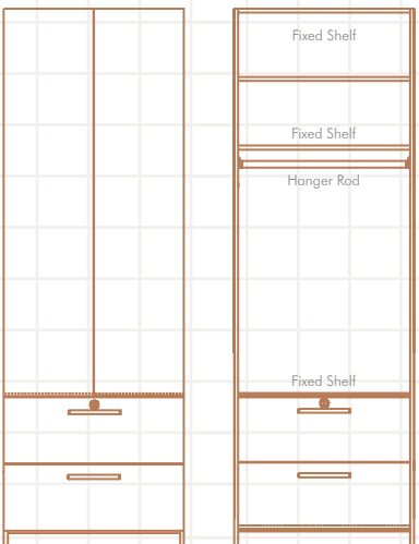
EXTERNAL 2 DRAWER W - 800,900,1000 D - 580 H - 1950 - 2100 - 2400
